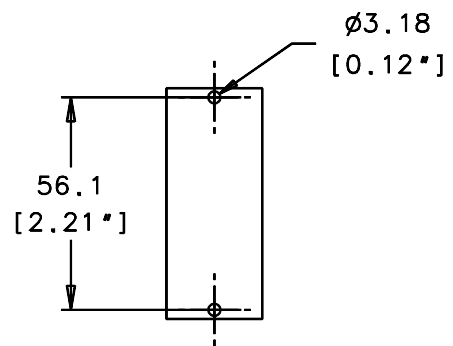
HOLE PATTERN
