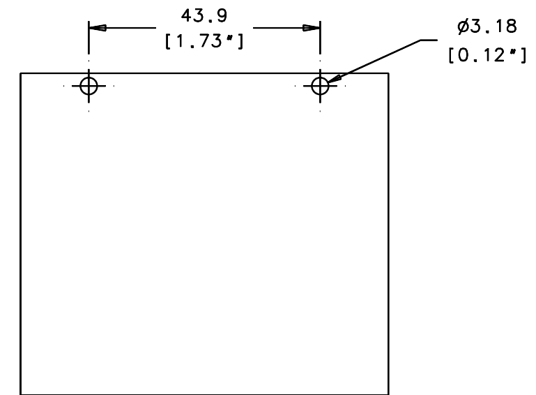
HOLE PATTERN
