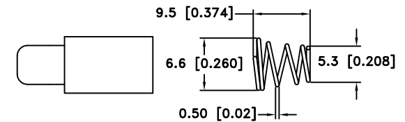
SPRING ORIENTATION VIEW
