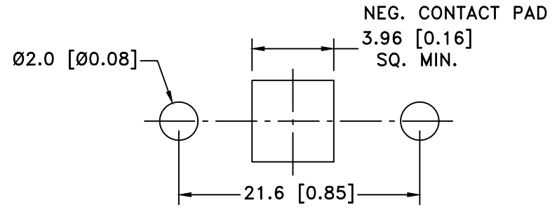
PCB LAYOUT
