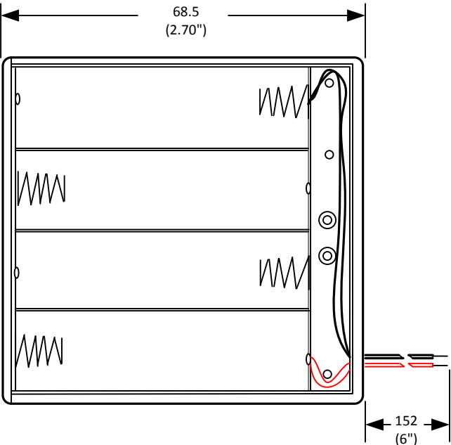
HOLDER
